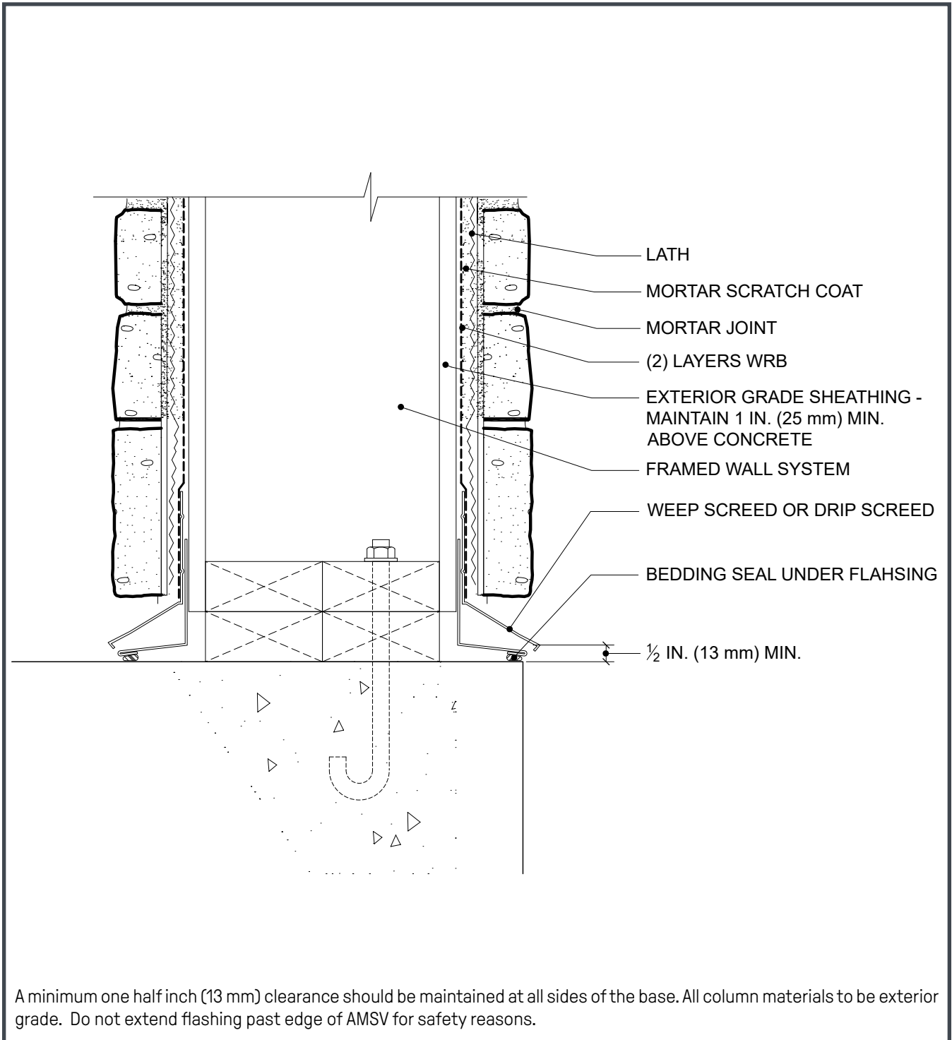
Figure 27. Column Base
